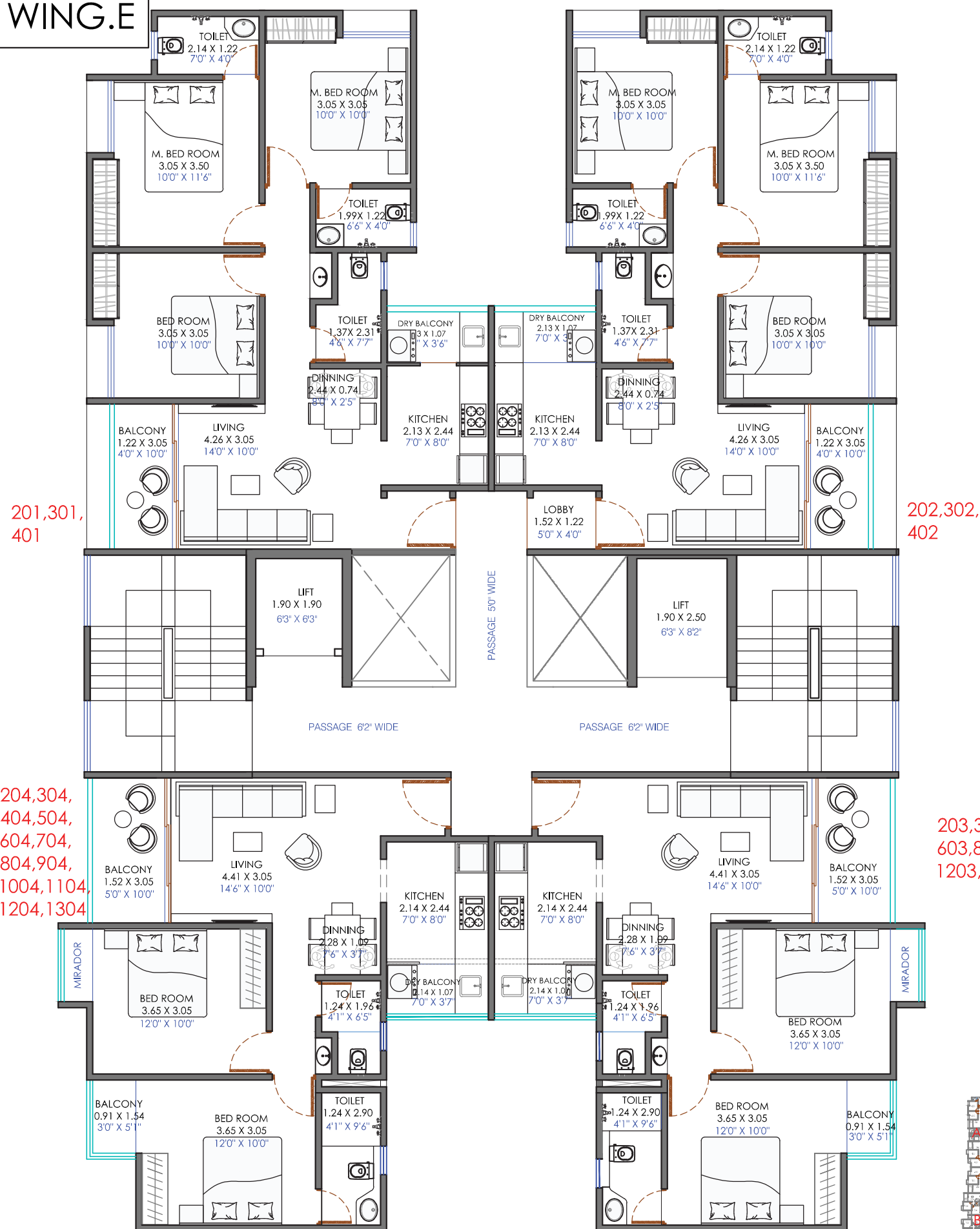
TYPICAL - 2ND,3RD,4TH,5TH,6TH,7TH,8TH,9TH,10TH,11TH,12TH,13TH FLOOR PLAN
