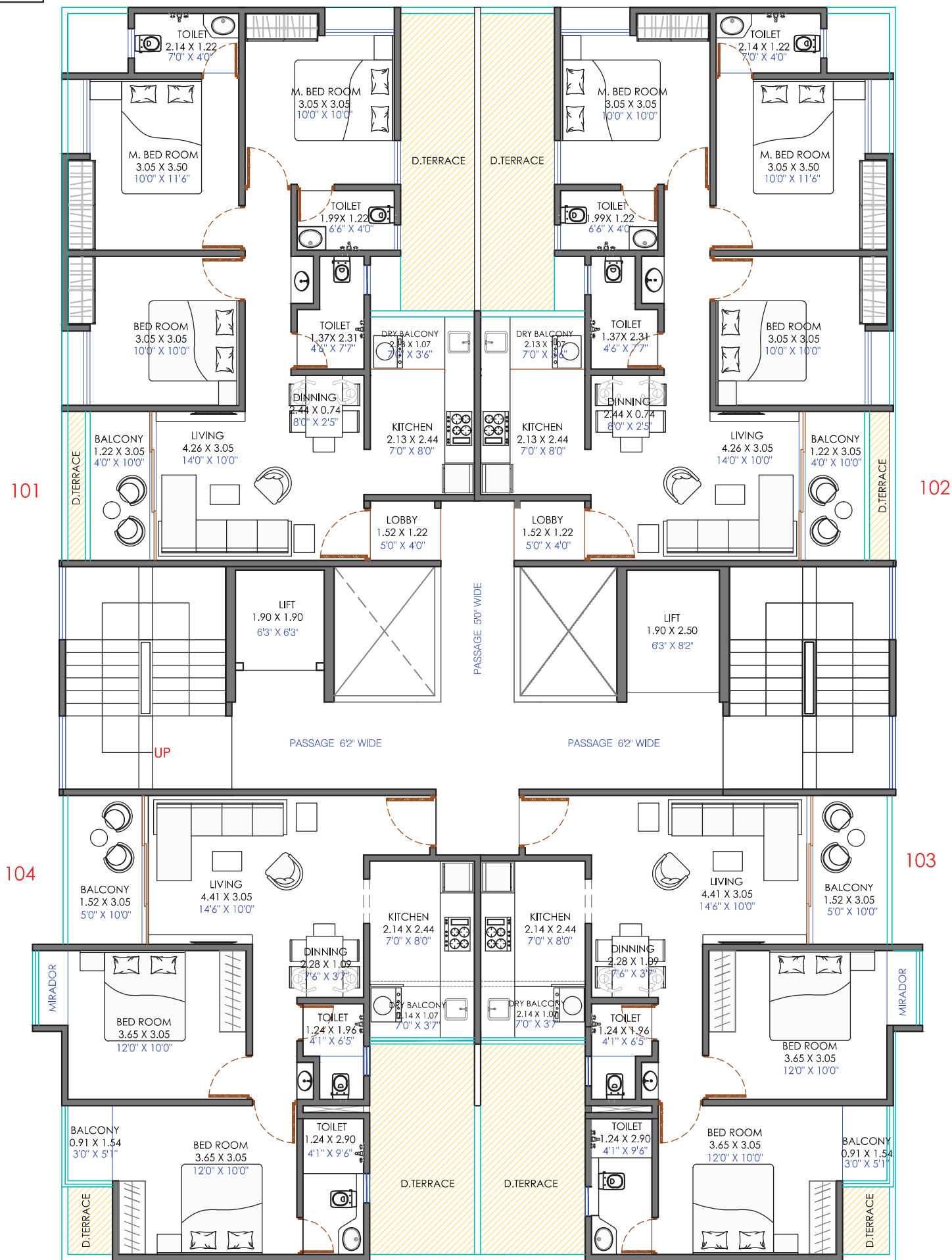
TYPICAL - 1ST FLOOR PLAN
