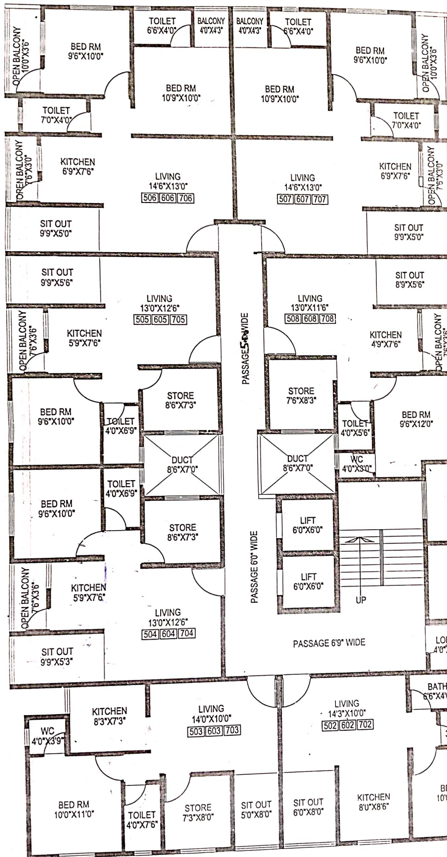
TYPICAL FLOOR PLAN (5th,6th,7th Floor Plan)
