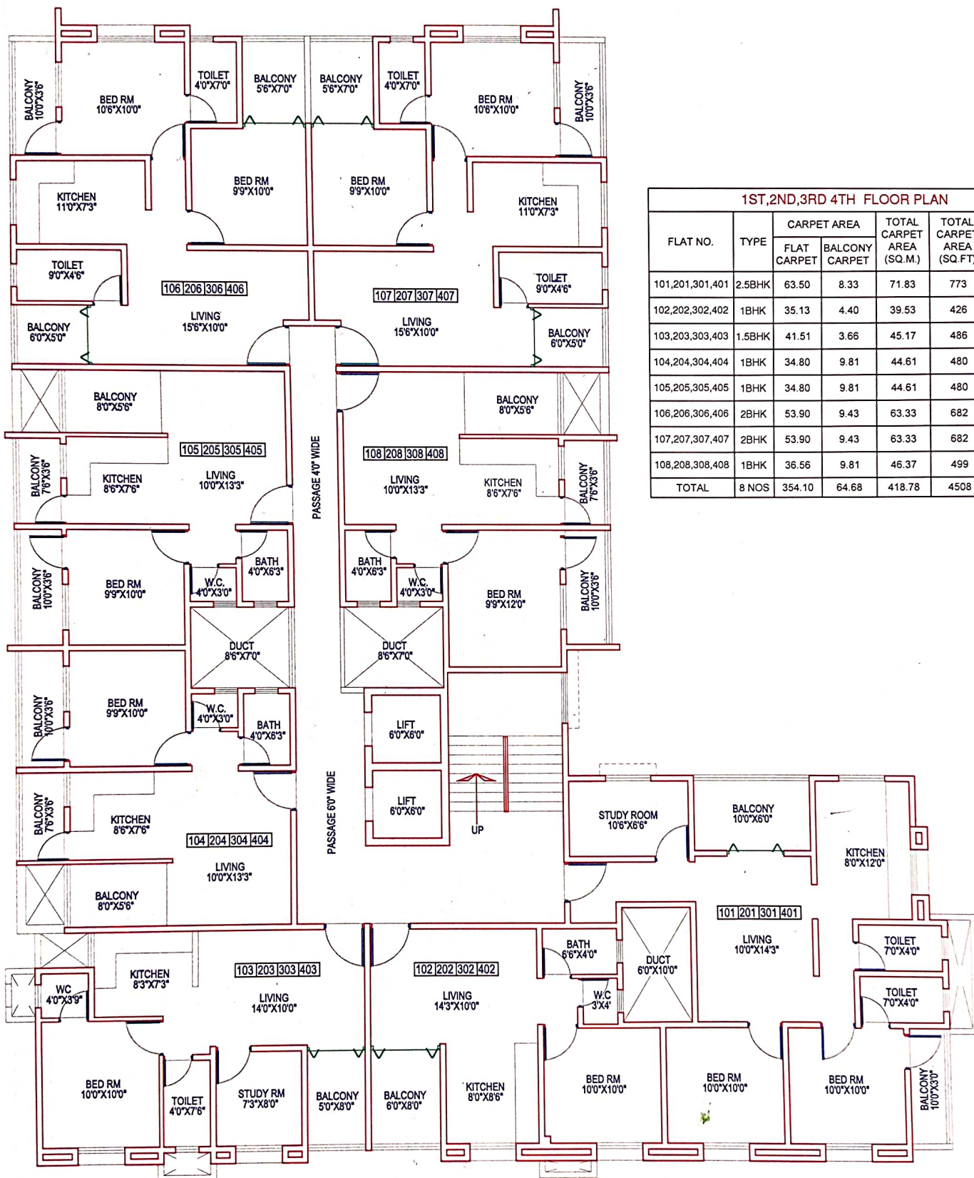
TYPICAL FLOOR PLAN 1ST TO 4TH
